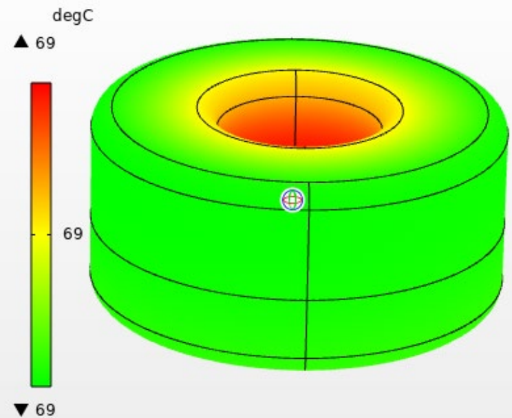
Lp=3.6 A, Ar=5 Slice: Temperature (degC)
