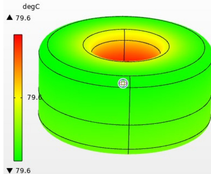
Lp=8.4 A, Ar=15 Slice: Temperature (degC)
