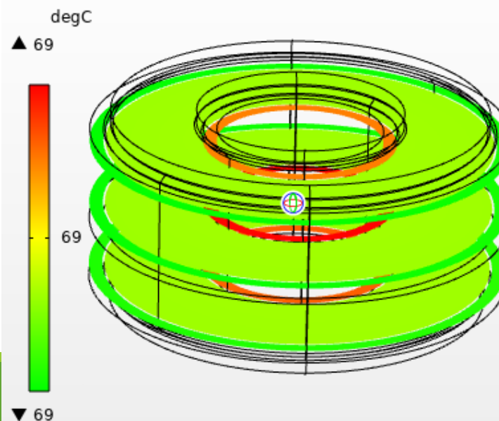
Lp=3.6 A, Ar=5 Slice: Temperature (degC)
